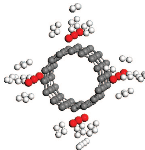
Figure 5. Schematic plots for the relaxed (\text{H}_2)_{32}/\text{Li}_8/\text{C}_{64} system, where all 32 \text{H}_2 molecules are located around the Li dopants. The red, gray, and white spheres represent Li, C, and H atoms, respectively.
