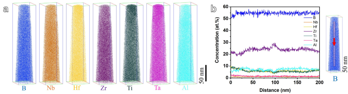
Fig. 4. Local chemical composition analysis of \text{MMB}_2 particle by APT. (a) The reconstruction of B, Nb, Hf, Zr, Ti, Ta, and Al atomic positions. (b) The corresponding composition profile from the cylindrical region indicated by the red arrow in the inset.
