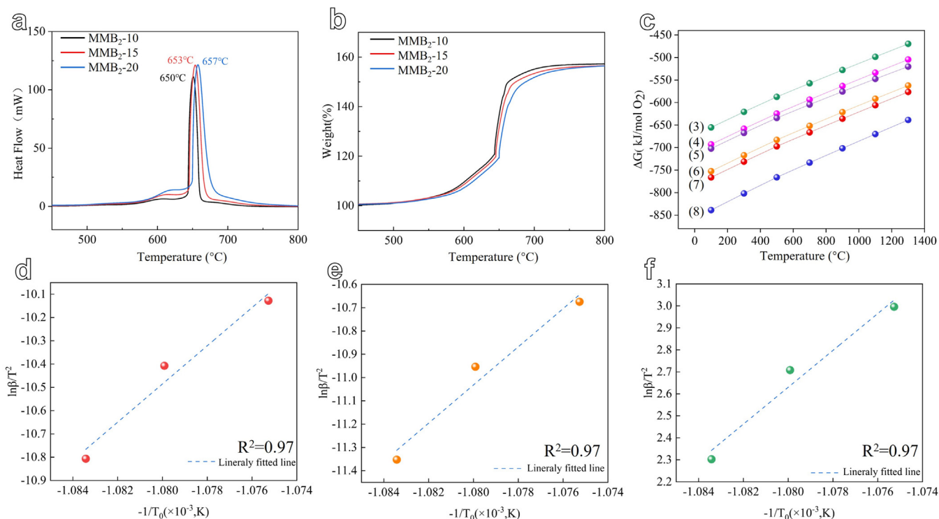
Fig. 9. (a, b) DSC curves and TG curves of MMB_2 at RT \sim 800 °C and different heating rates; (c) Thermodynamic analysis of the Reactions (3–8); (d–f) Plots of Kissinger model, Flynn-Wall-Ozama model and Starink model respectively.
