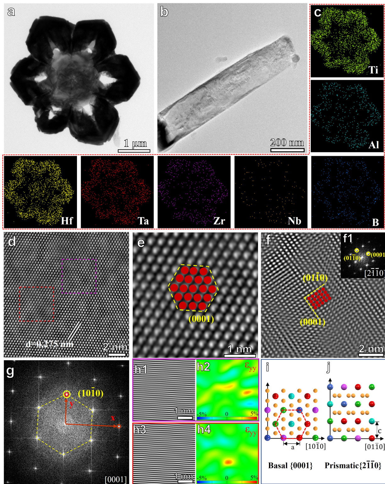
Fig. 3. (a) HRTEM graph of MMB_2 particle, the electron beam is parallel to the [0001] zone. (b) HRTEM graph of another MMB_2 particle, the electron beam is parallel to the [2\bar{1}10] zone. (c) The corresponding EDS compositional maps of (a). (d) High-resolution transmission electron microscope (HRTEM) graph of MMB_2 particle and the electron beam is parallel to the [0001] zone, the red and purple squares show the lattice distortion region. (e) HRTEM image at a higher magnification, showing the atomic configuration of (0001) plane. (f) HRTEM graph of another (HfTaZrNbTi)_2B_2 particle along [2\bar{1}10] direction and (01\bar{1}0) and (0001) planes are indexed. (f1) the corresponding FFT pattern. (g) FFT pattern of Fig. 2(a). (h1, h3) The IFFT image shows perfect periodicity with noticeable lattice distortion. (h2, h4) GPA mapping showing an overall strain field at nanoscale. The color scale represents change in strain intensity from -5\% (compressive) to 5\% (tensile). (i, j) Schematic illustration of the atomic structure of the MMB_2 .
