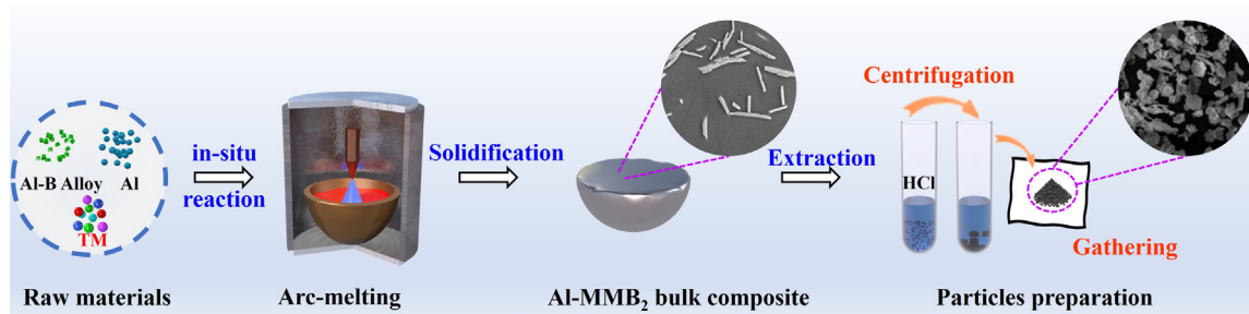
Fig. 1. The fabrication process of the Al-MMB 2 bulk composites and MMB 2 particles.
