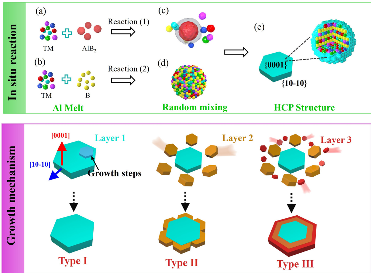
Fig. 5. Schematic illustration of the in-situ reaction and growth mechanism of the MMB 2 microcrystals in the Al melt.
